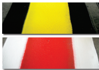
H18 at Royal Air Force/UK equipped with 1-component cold paint Airless system (two pumps) with 90 cm wide line marker unit incl. 4 paint and glass bead guns as well as 3 paint- and glass bead guns for taxiways (black/yellow/black), 2 x 225 l pressurised container
