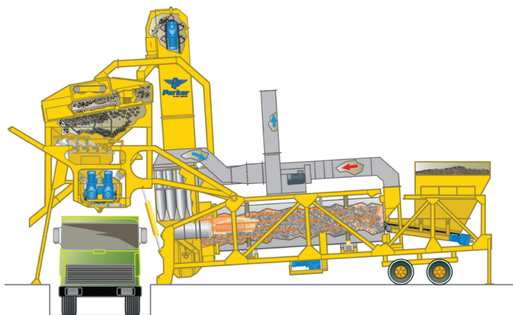
Option 1: Super-Roadmix with combined 2 bin compartment feed unit
