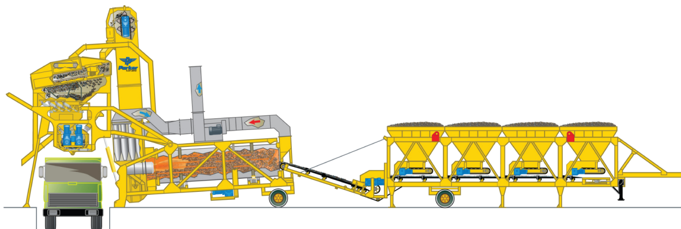
Option 2:* Super-Roadmix complete with separate three or four bin mobile feed unit
